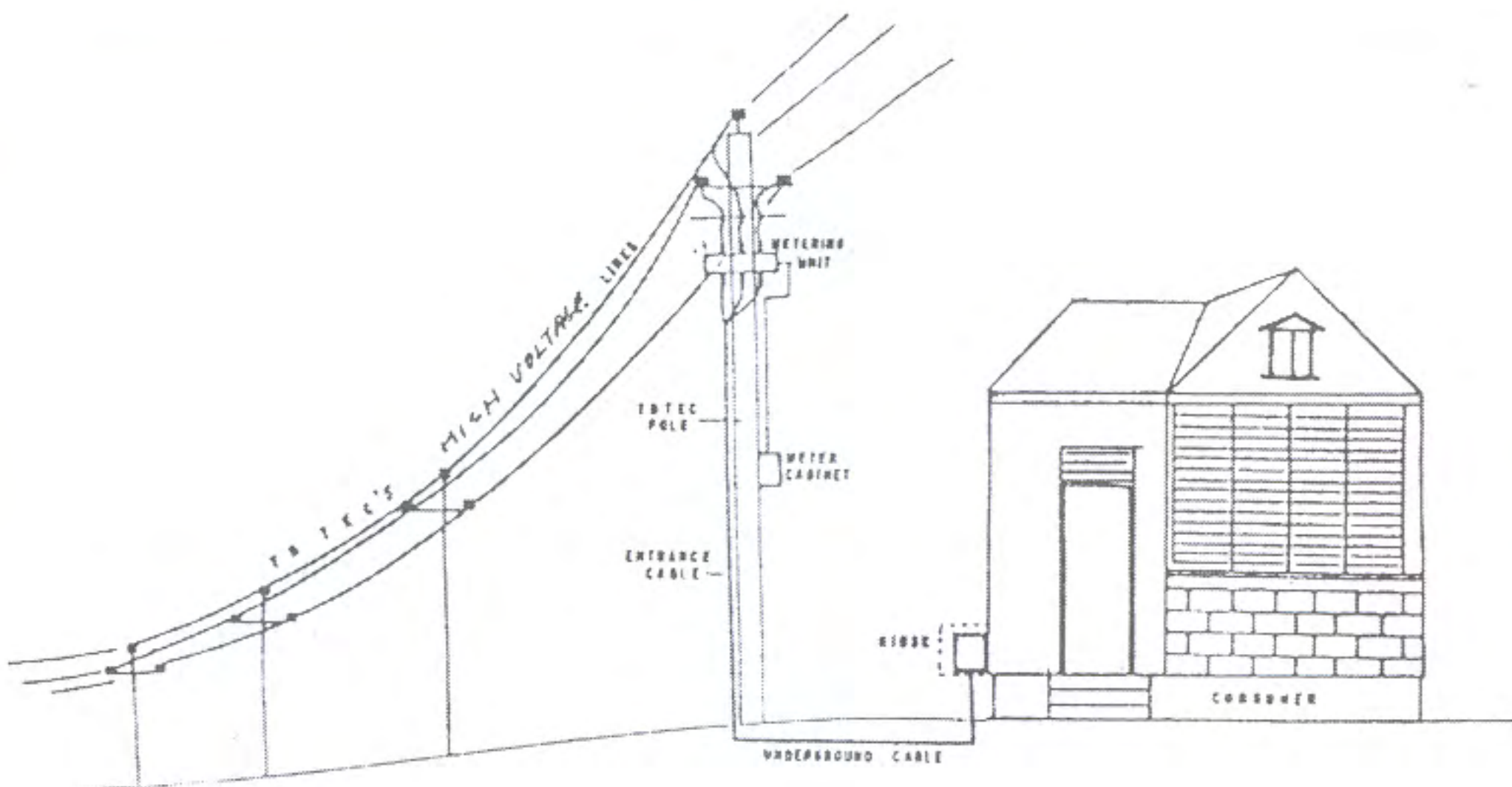
TYPICAL INSTALLATION Single Metered High Voltage Supply
