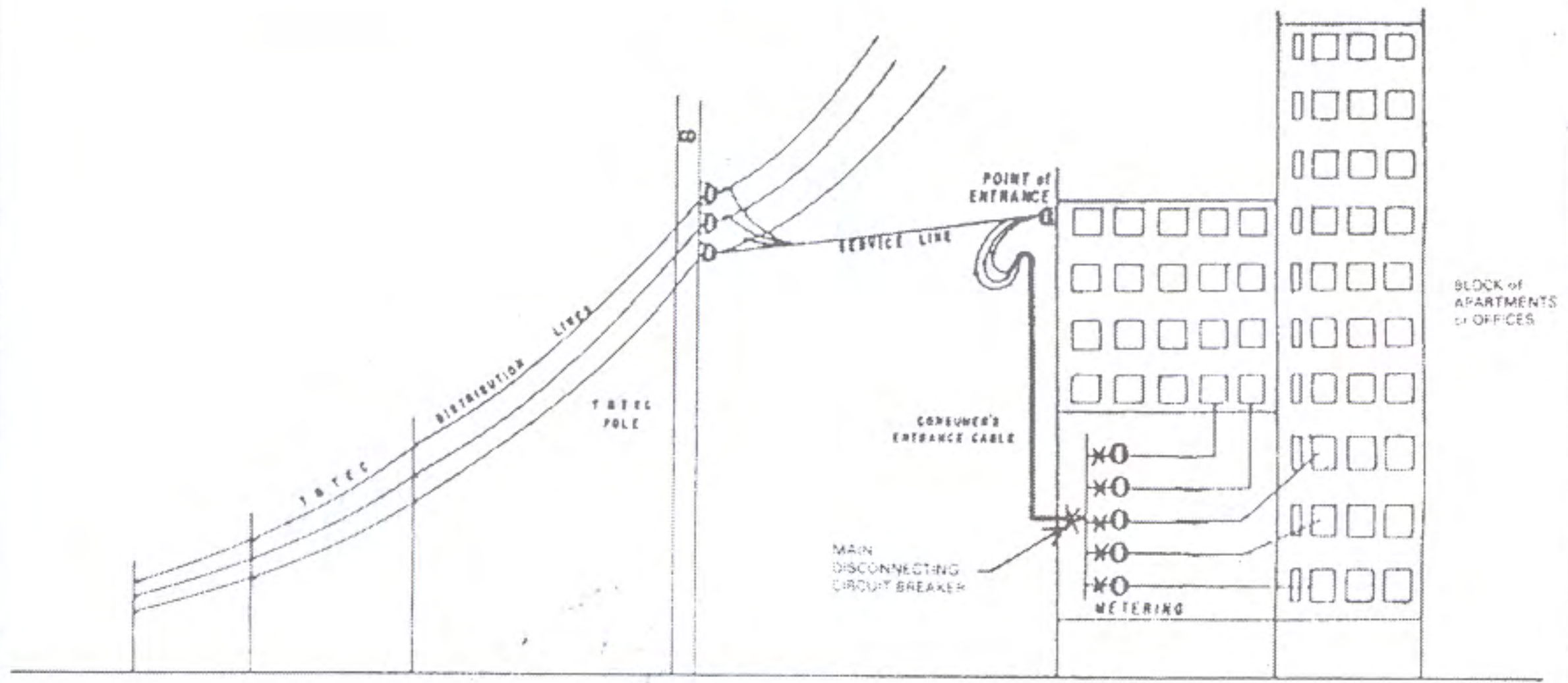
TYPICAL INSTALLATION Multi-Metered Low Voltage Supply (7 meters or less)
