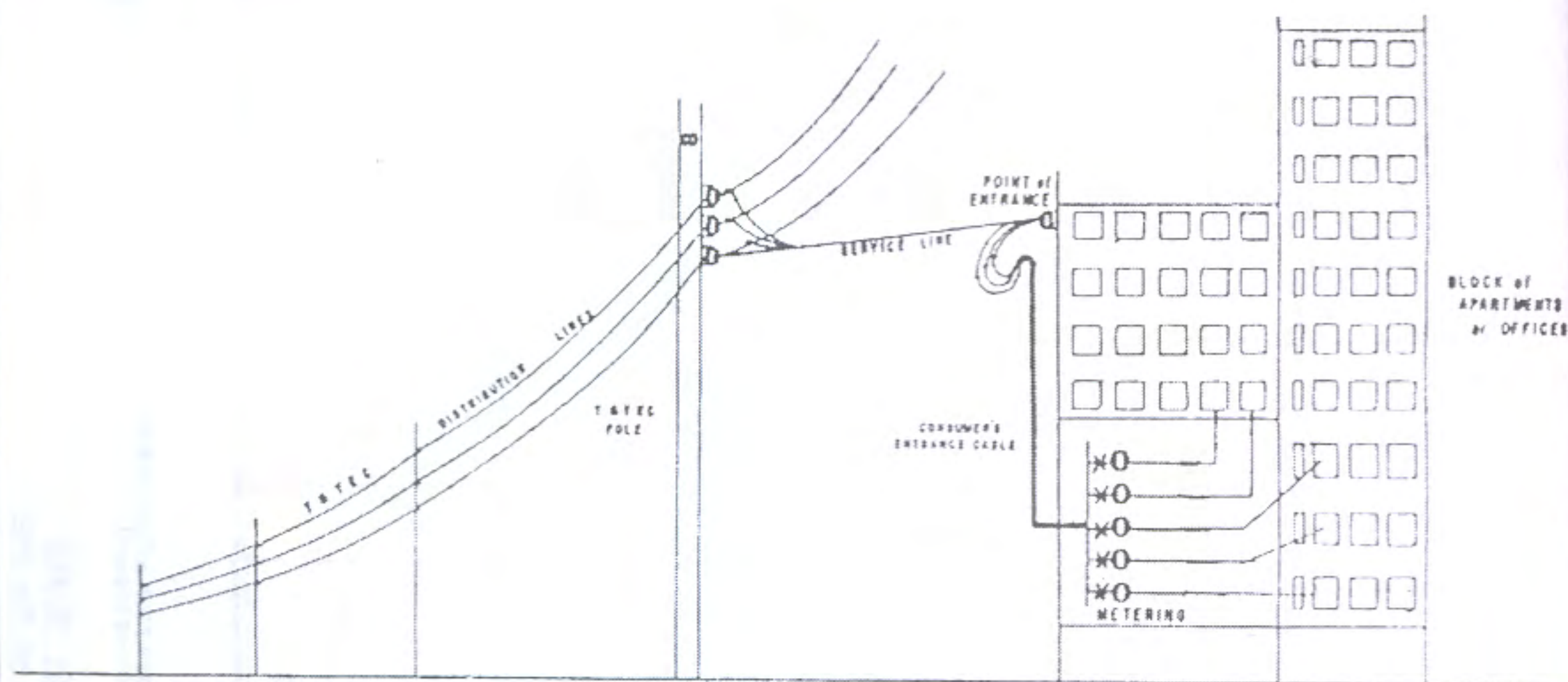
TYPICAL INSTALLATION Multi-Metered Low Voltage Supply (6 meters or less)
